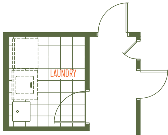
OPT. LAUNDRY ROOM (TO REPLACE LOFT AREA)
