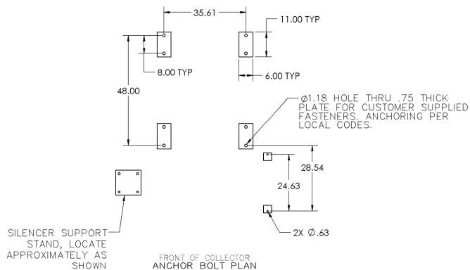
FRONT OF COLLECTOR ANCHOR BOLT PLAN
