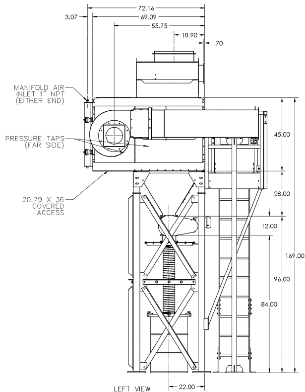
LEFT VIEW
