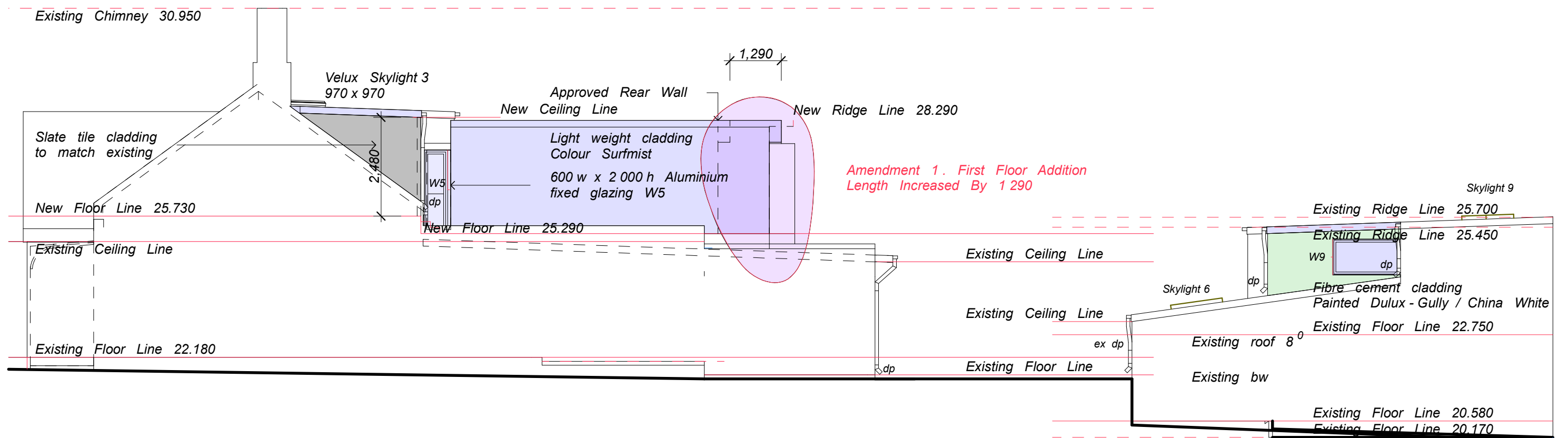
NORTH ELEVATION
