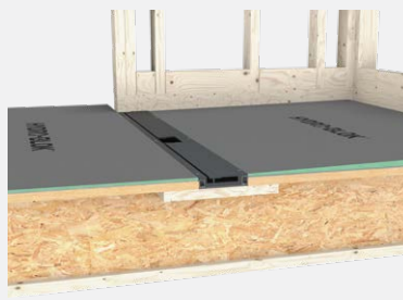
THIN Single Slope Shower Pans
