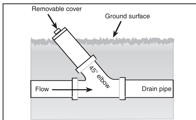
Figure 4b. PVC pipe cleanout for drain pipe.
