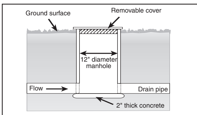
Figure 4a. Manhole cleanout for drain pipe.
