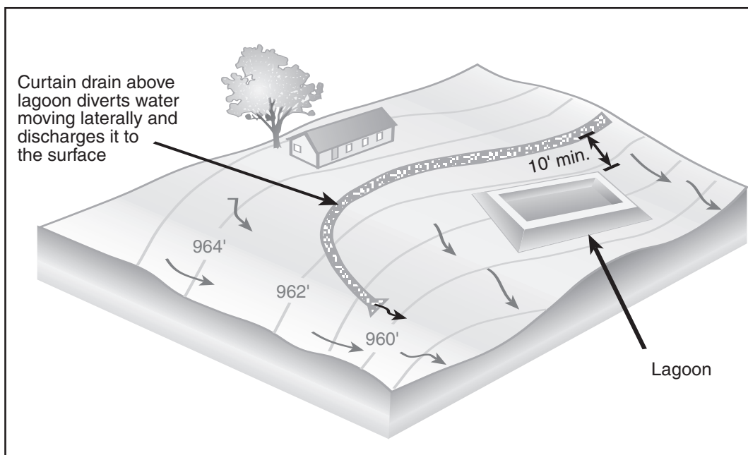
Figure 7a. View of curtain drain location.
