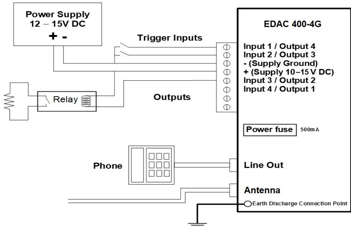
Figure 1: Typical EDAC 400-4G Installation
