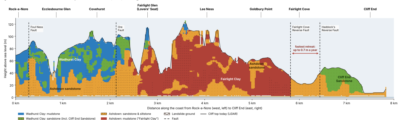
Figure 2.2. The rocks behind the cliffs. Brown areas are the soft Ashdown mudstones ("Fairlight Clay"), orange the stronger Ashdown sandstones and siltstones, green and yellow the Wadhurst Clay. Black lines are faults; hatched patches are mapped landslides. The dotted sea area is classed by the British Geological Survey as rock and hard seabed. Based upon Data provided by the British Geological Survey © UKRI. All rights reserved. LiDAR: Environment Agency, Open Government Licence.
