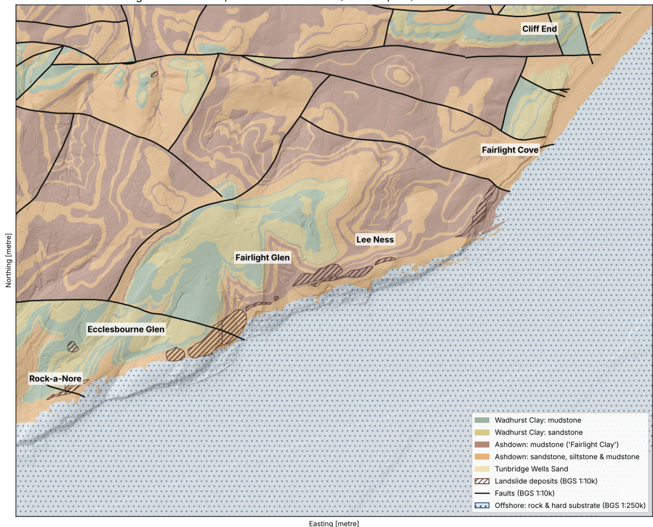
The rocks of the Hastings cliffs: bedrock, faults and landslides (BGS 1:10,000)
