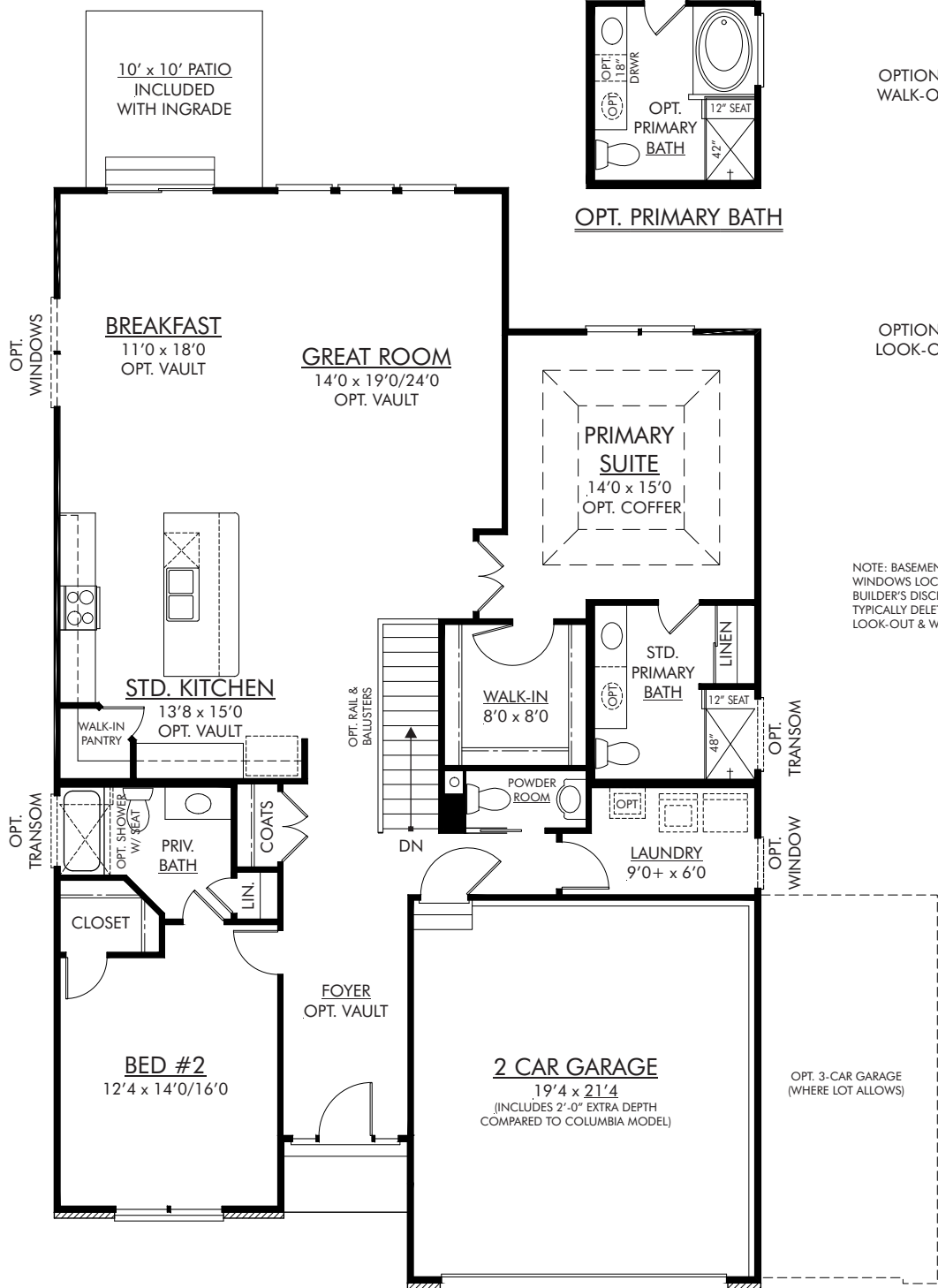
FIRST FLOOR PLAN 1,826 SqFt - DRAWN PER ELEVATION B
