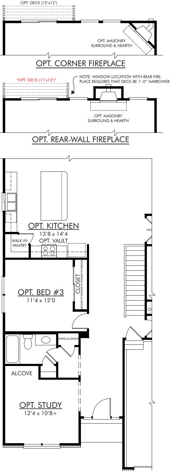
OPT. STUDY, OPT. BEDROOM, OPT. KITCHEN, & OPT. "L" STAIRCASE (KITCHEN, STUDY, BED #3, AND STAIRCASE OPTIONS ARE SEPARATE FROM EACH OTHER AND MAY BE ADDED IN ANY COMBINATION)
