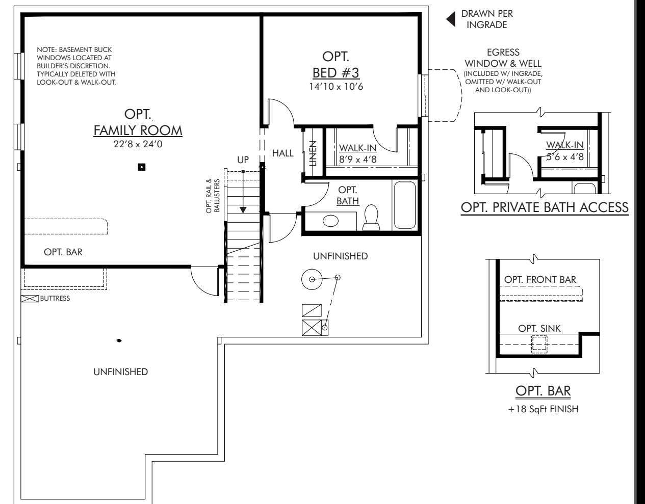
OPT. LOWER LEVEL PLAN
