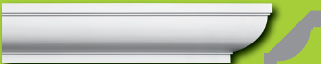
MD 1890 • 6 1/2" Projection • 7" Height • 12'0" Length
