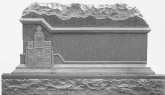
Die: 72"wx12"dx36"h (P5) Base: 78"wx16"dx10"h (P1) w/2" Pol Margin
