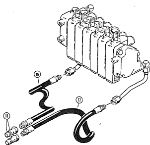
D100 Connecting Hyd. For 150M, 170, 180, 190 & 1500 Series Uni-Loaders Without Flow Control Valve
