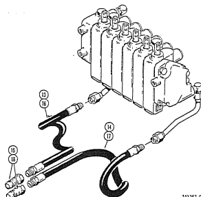
D100 Connecting Hyd. For 1030 Uni-Loaders & 150M, 170, 180, 190, & 1500 Series Without Flow Control Valve
