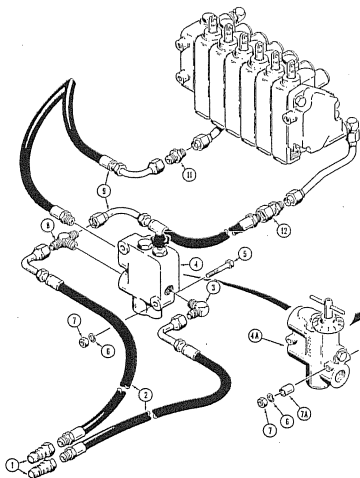
D100 Connecting Hyd. For 150M, 170, 180, 190 & 1500 Series Uni-Loaders Without Flow Control Valve
