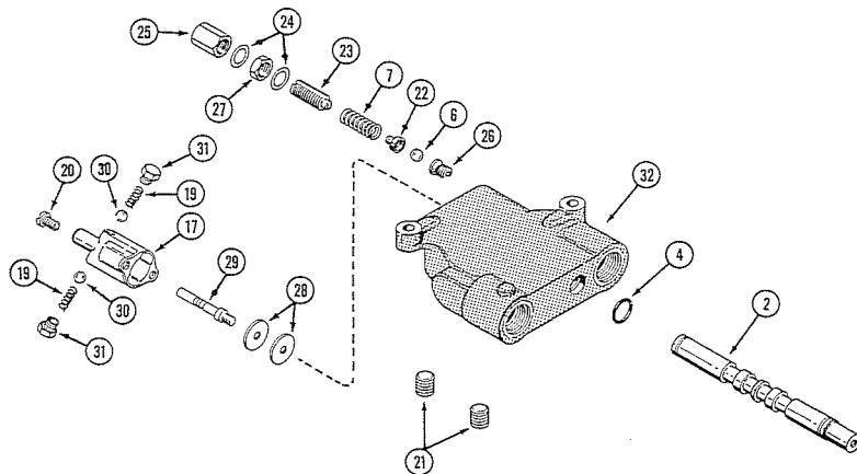
SINGLE SPOOL VALVE (Tractors with Manual Lift)
