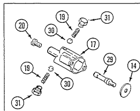
TRAVEL SECTION DETENT GROUP
