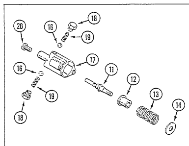
LIFT SECTION DETENT GROUP
