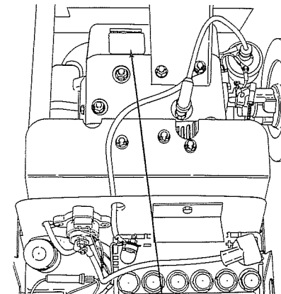
ENGINE MODEL, SERIAL AND SPECIFICATION NUMBER
