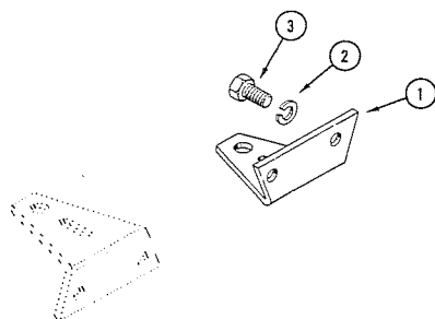
MOUNTING POSITION FOR 220, 222 AND 224 TRACTORS.
