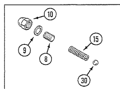
LIFT SECTION RELIEF GROUP
