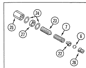
TRAVEL SECTION RELIEF GROUP
