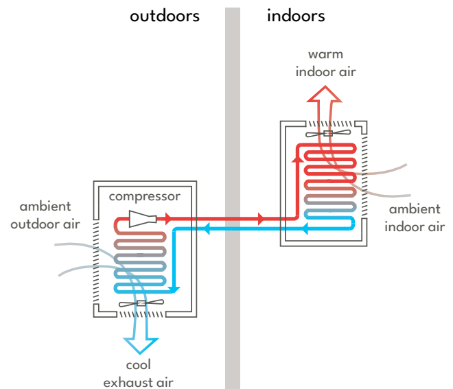
Fig 1. In heating mode, mini-splits transfer heat from outside to inside via refrigerant lines. Heat from air drawn through the outdoor unit is transferred to a refrigerant, which is pumped through a compressor to the indoor unit. Heat from the refrigerant is then transferred to ambient indoor air to produce warm air. In cooling mode, mini-splits operate in reverse, moving heat from inside to outside.
