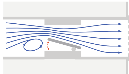
Fig 2. A Constant Airflow Regulator (CAR) automatically dampens airflow to achieve consistent ventilation.
