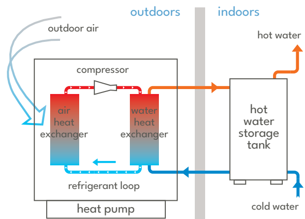
Fig 1. Heat from outdoor air is drawn into the AWHP and is absorbed by a refrigerant. As the refrigerant passes through the compressor, its pressure and temperature rises. The refrigerant then passes through the water heat exchanger to heat the domestic supply water, which is pumped to the storage tank for distribution.
