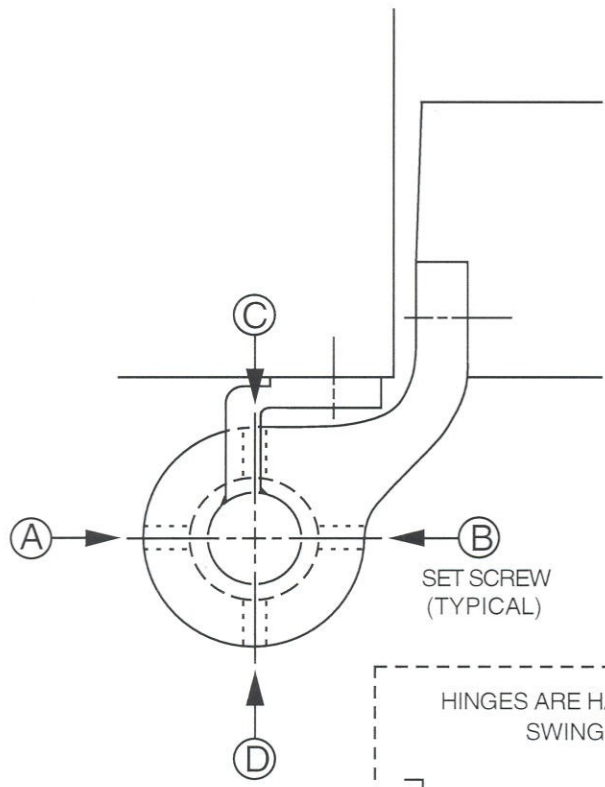
SH-460 HINGE (HALF-MORTISE)
