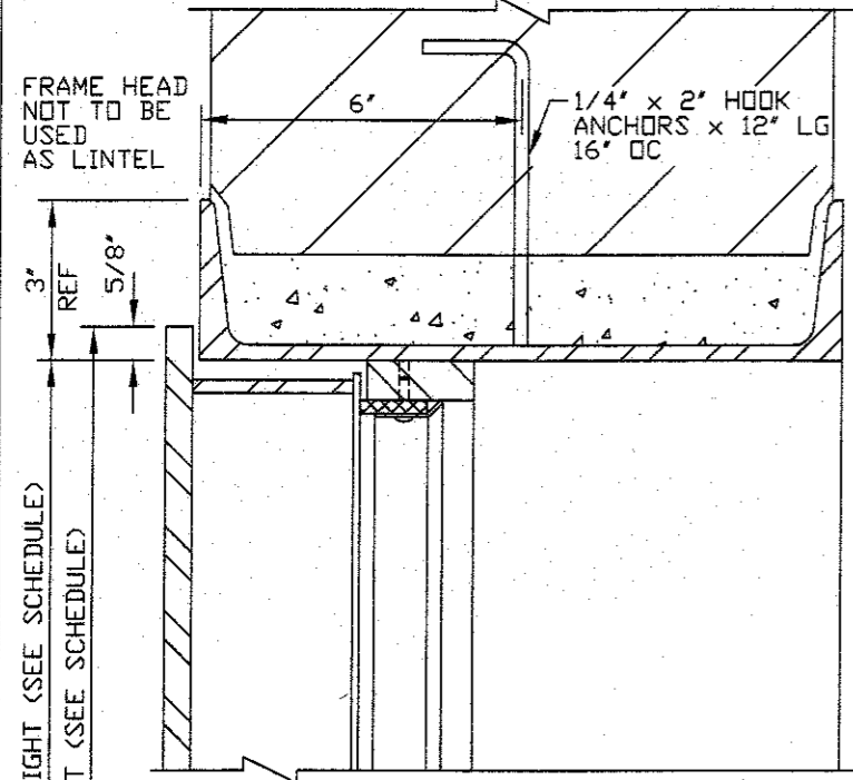
HEAD SECTION 3
