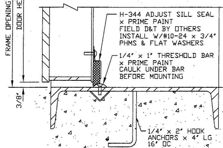
SILL SECTION 4
