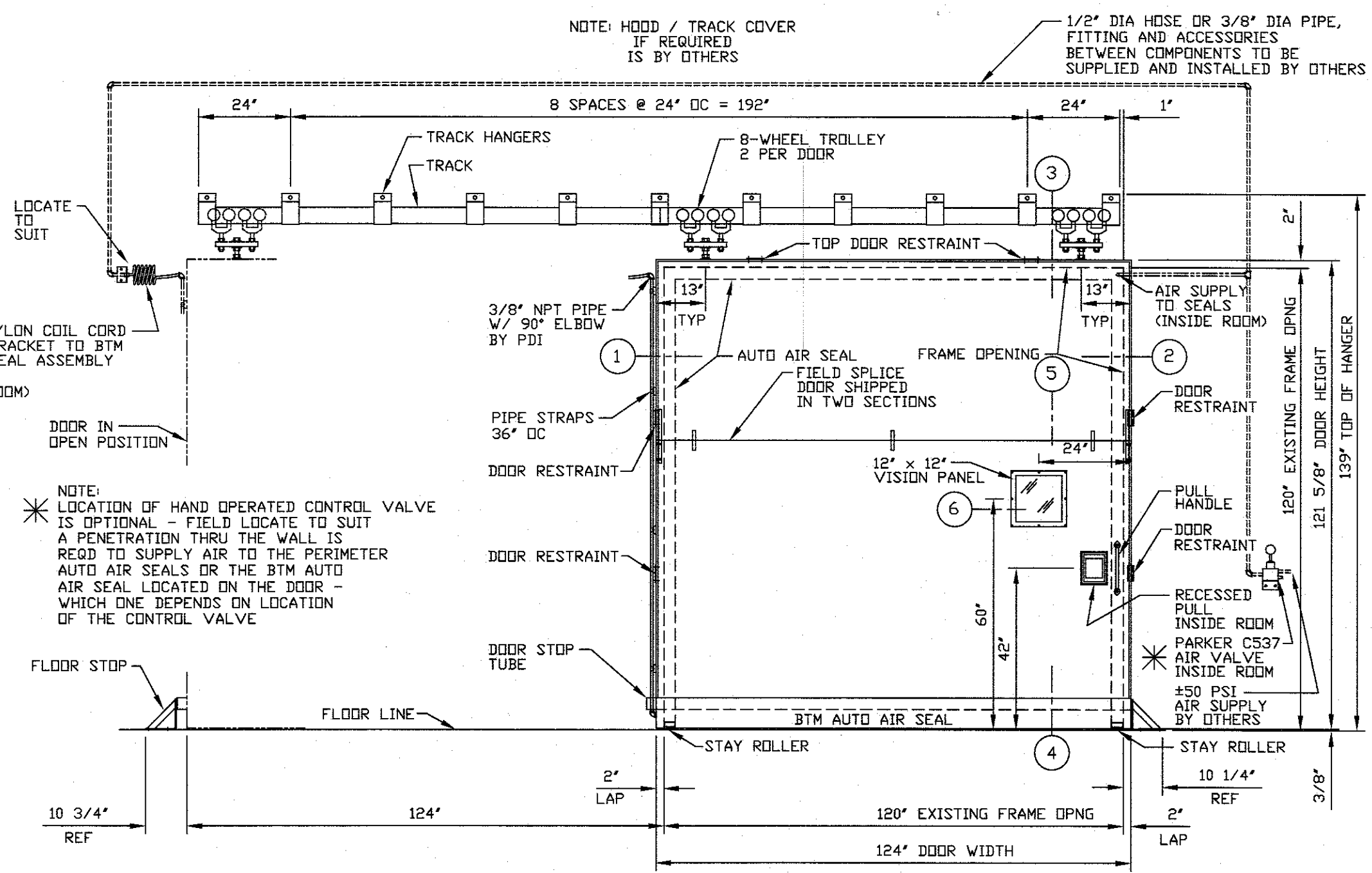
ELEVATION A (1) REQD LH SLIDE SHOWN RH SLIDE OPPOSITE DOOR WEIGHT: APPROX 1950 LBS
