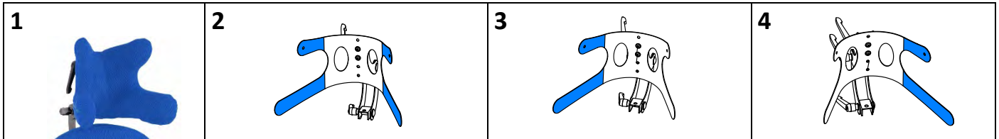
1 Butterfly headrest 22 cm x 18 cm / 8.6" x 7" 2 Headrest enlarged on both sides Up horn + 5 cm / +1.9" Bottom horn + 7 cm / +2.7" 3 Headrest right side enlarged Up horn + 5 cm / +1.9" Bottom horn + 7 cm / +2.7" 4 Headrest left side enlarged Up horn + 5 cm / +1.9" Bottom horn + 7 cm / +2.7"
