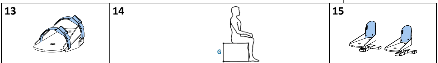
13 Feet straps (set of 4 pcs.) 14 Foot platforms height adjustment Range 1 Range 2 Range 3 14 Dimension G 12 - 30 / 4.7"- 11.8" 16 - 33 / 16"- 6.3" 26 - 44 / 10.23" - 17.3" 15 3D Foot platforms with heel supports Heel supports height: 12 cm
