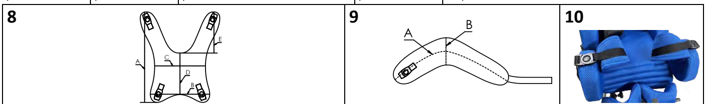
8 Vest S A - 26 cm / 10.2" B - 17 cm / 6.6" C - 14 cm / 5.5" D - 8,5 cm / 3.3" E - 15 cm / 5.9" 8 Vest M A - 31 cm / 12.2" B - 20 cm / 7.8" C - 16 cm / 6.2 " D - 8,5 cm / 3.3" E - 19 cm / 7.4" 8 Vest L A - 39 cm / 15.3" B - 25 cm / 9.8" C - 20 cm / 7.8" D - 8,5 cm / 3.3" E - 29 cm / 11.4" 9 Pelvic belts S: A - 31 cm / 12.2" B - 8 cm / 3.1" 9 Pelvic belts M: A - 35 cm / 13.77" B - 8 cm / 3.1" 9 Pelvic belts L: A - 45 cm / 17.7" B - 10 cm / 3.9" 10 Legs abduction belts
