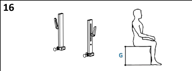
Feet platforms height adjustment
