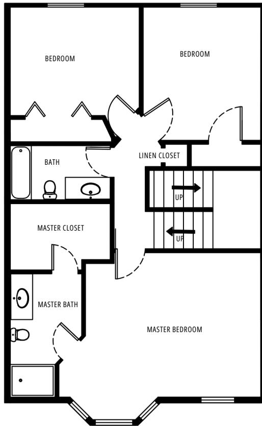
SECOND FLOOR
