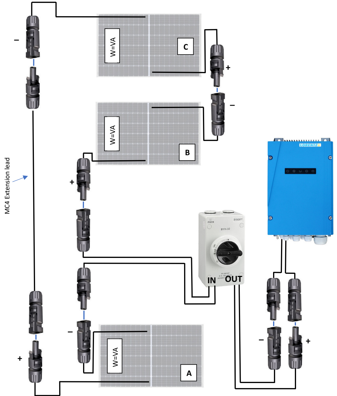
3S1P V2.0 wiring diagram SWP
