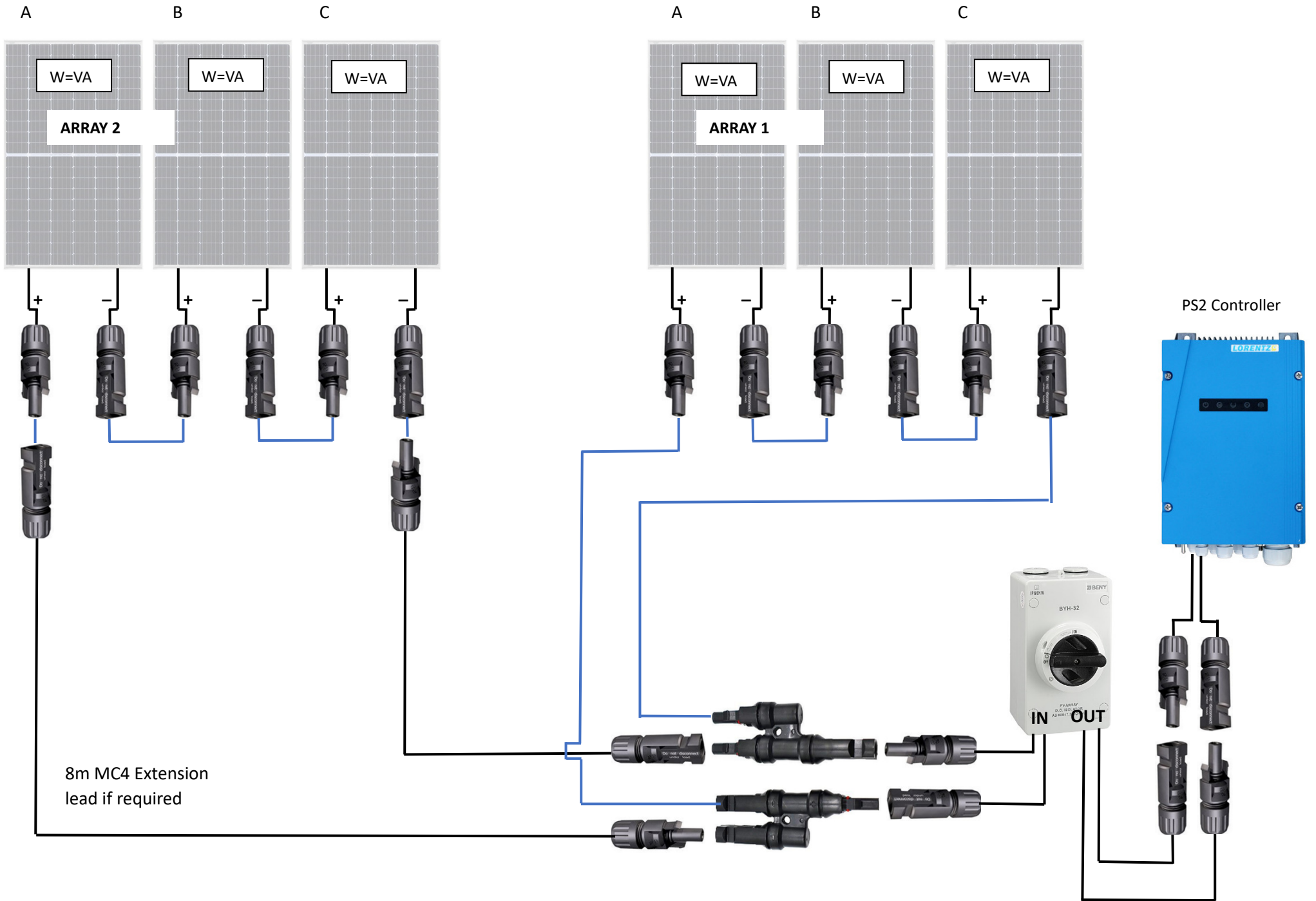
3S2P V2.0 wiring diagram SWP
