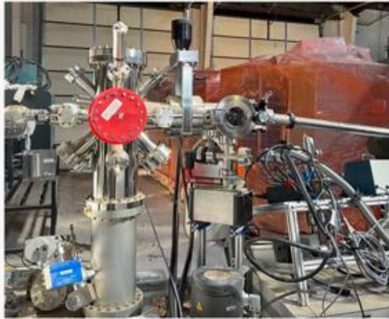
Ultra-High Vacuum System- For Simulated Space Environments (UHV) $50,000 OBO
