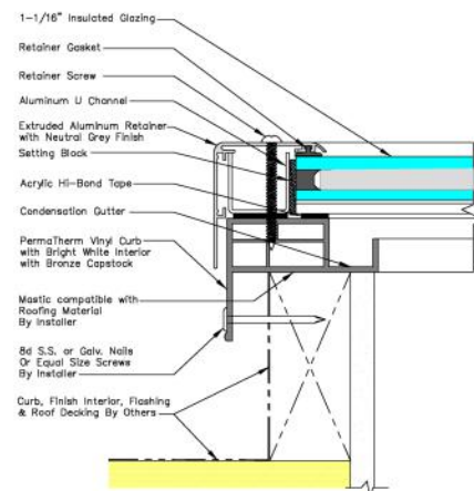
DETAIL 1
