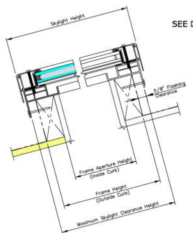
VERTICAL CROSS SECTION
