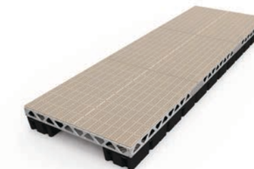
8' X 24' COMPLETE FLOATING DOCK KIT 1025 lbs / 465 kg (w/o decking - 725 lbs / 329 kg)
