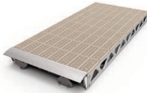
4' X 8' COMPLETE RAMP KIT 120 lbs / 54 kg (w/o decking - 70 lbs / 31 kg)
