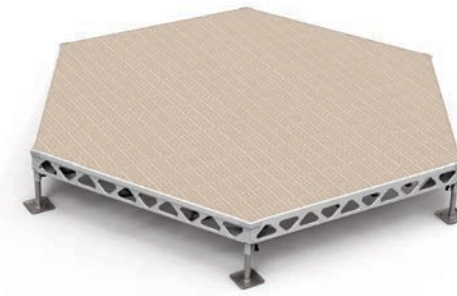
14' x 16' COMPLETE HEXAGON STANDING DOCK KIT 1' - 2' LEGS 665 lbs / 301 kg (w/o decking - 365 lbs / 165 kg)
