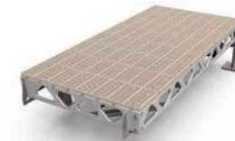
4' x 8' COMPLETE QUICK LINK DOCK KIT 1' - 2' LEGS 130 lbs / 59 kg (w/o decking - 80 lbs / 36 kg)
