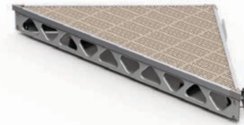
8' COMPLETE CORNER KIT 70 lbs / 32 kg (w/o decking - 45 lbs / 20 kg)
