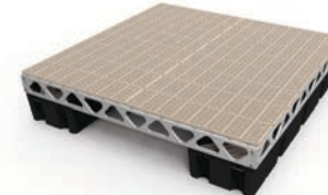
8' X 8' COMPLETE FLOATING DOCK KIT 330 lbs / 150 kg (w/o decking - 230 lbs / 104 kg)
