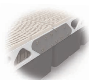
FLOATING DOCK CONNECTOR KIT Connects 4' x 8' and 8' x 8' floating docks together to create a rigid floating dock.
