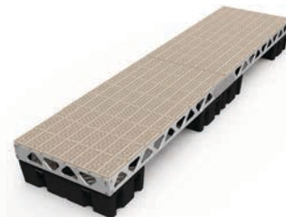
4' X 16' COMPLETE FLOATING DOCK KIT 380 lbs / 172 kg (w/o decking - 280 lbs / 127 kg)
