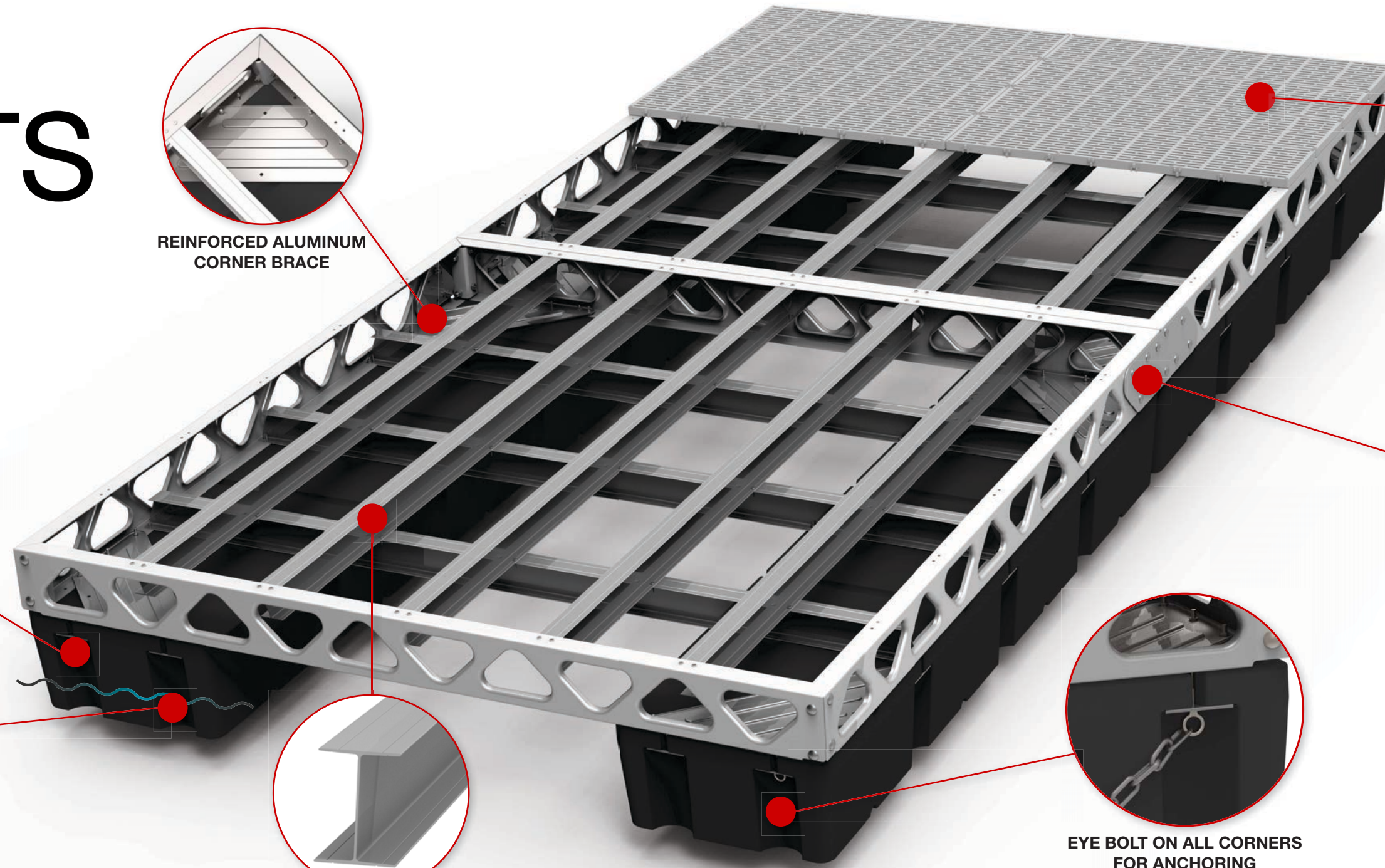
ALUMINUM I JOISTS ON 16" CENTERS
