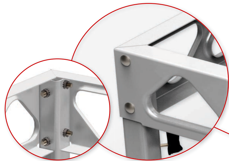
BOLT TOGETHER MARINE GRADE ALUMINUM FORMED FRAME
