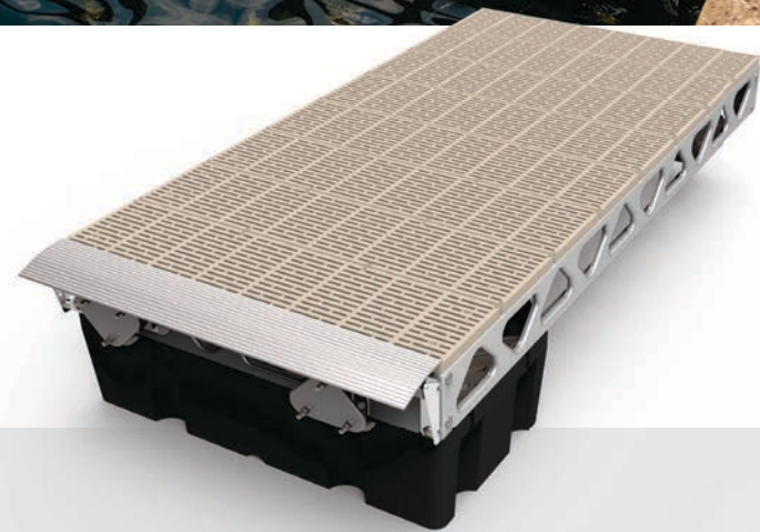
4' x 8' COMPLETE FLOATING RAMP KIT
