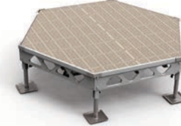
7' x 8' COMPLETE HEXAGON STANDING DOCK KIT 1' - 2' LEGS 220 lbs / 100 kg (w/o decking - 120 lbs / 54 kg)
