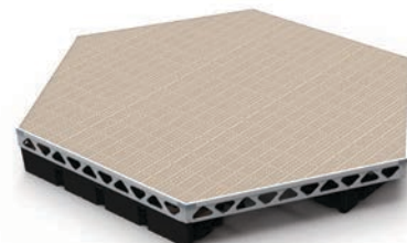
14' x 16' COMPLETE HEXAGON FLOATING DOCK KIT 920 lbs / 417 kg (w/o decking - 620 lbs / 281 kg)
