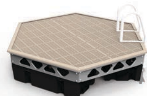
7' x 8' COMPLETE HEXAGON FLOATING DOCK KIT 315 lbs / 143 kg (w/o decking - 215 lbs / 97 kg)
