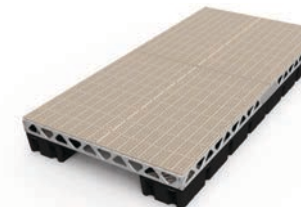
8' X 16' COMPLETE FLOATING DOCK KIT 680 lbs / 308 kg (w/o decking - 480 lbs / 218 kg)
