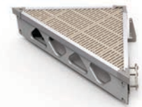
4' COMPLETE CORNER KIT 30 lbs / 13 kg (w/o decking - 17 lbs / 6 kg)
