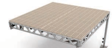
4' x 8' COMPLETE QUICK LINK DOCK KIT 4' - 8' LEGS 145 lbs / 66 kg (w/o decking - 95 lbs / 43 kg)
