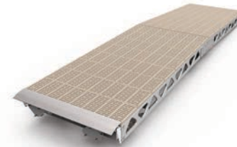
4' X 16' COMPLETE RAMP KIT 260 lbs / 118 kg (w/o decking - 160 lbs / 72 kg)
