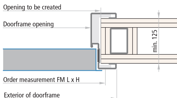
Door cross section and plasterboard version: REI 120 EI 2 60 - EI 2 120
