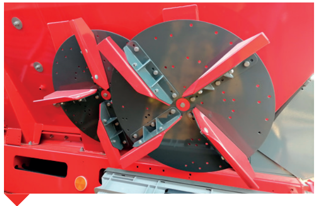
Discs for spreading lime
