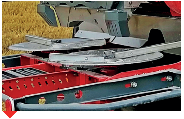
Discs for granulated fertilisers
