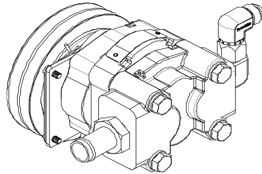
PU-SP4-11 2 GROOVE, SIDE PORT
