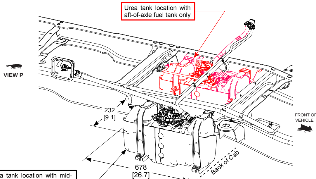
NARROW FRAME CHASSIS CAB
