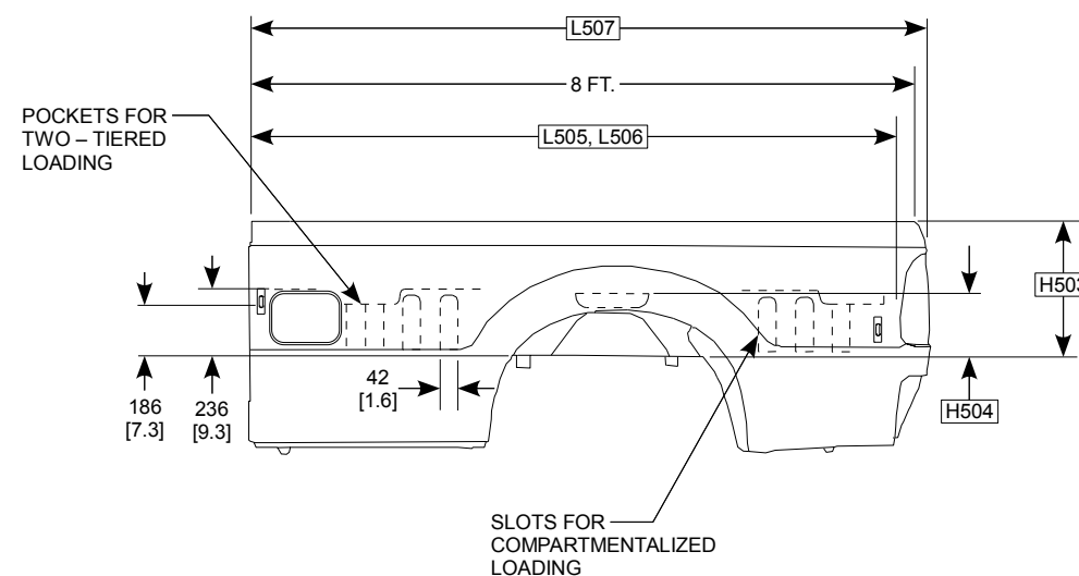
8 FT. BOX
