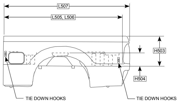
6 3/4 FT. BOX
