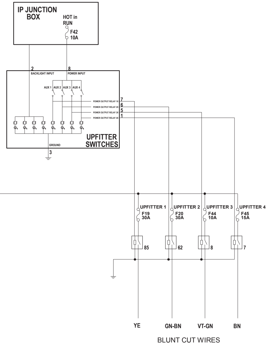
CUSTOMER ACCESS (UPFITTER) SCHEMATIC
