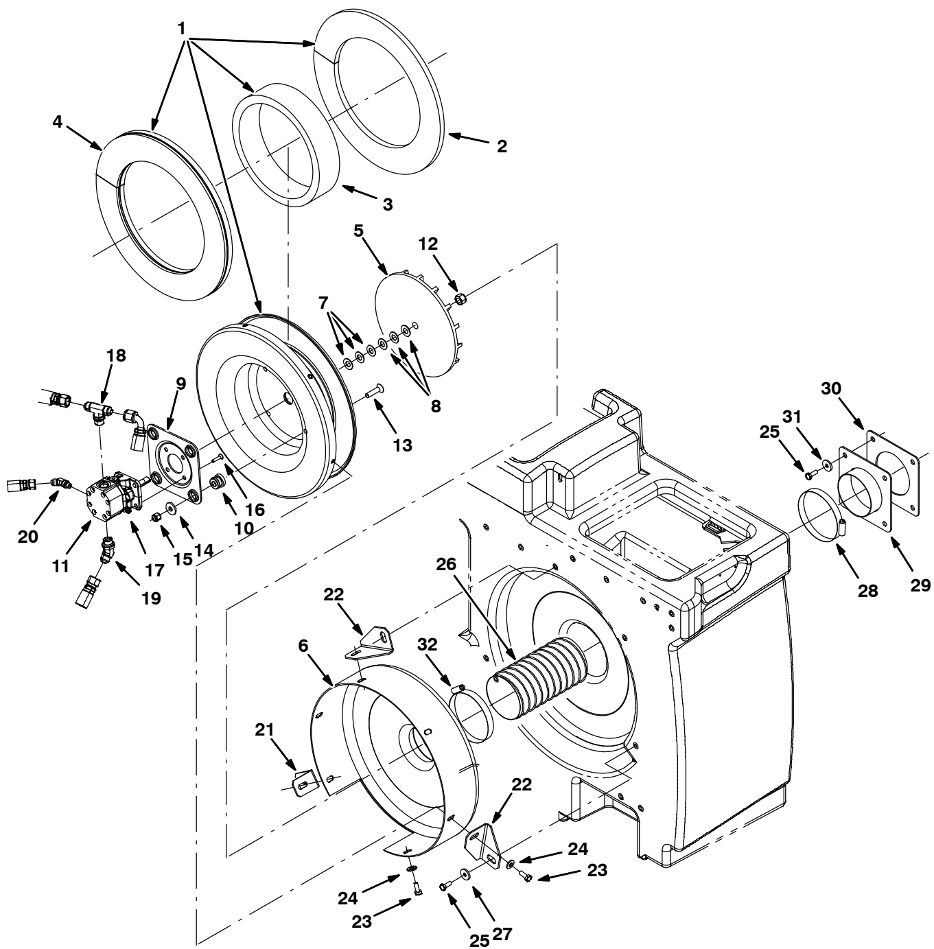
Fig. 48 – Vacuum Fan Group, Scrubbing (0000–0778)
