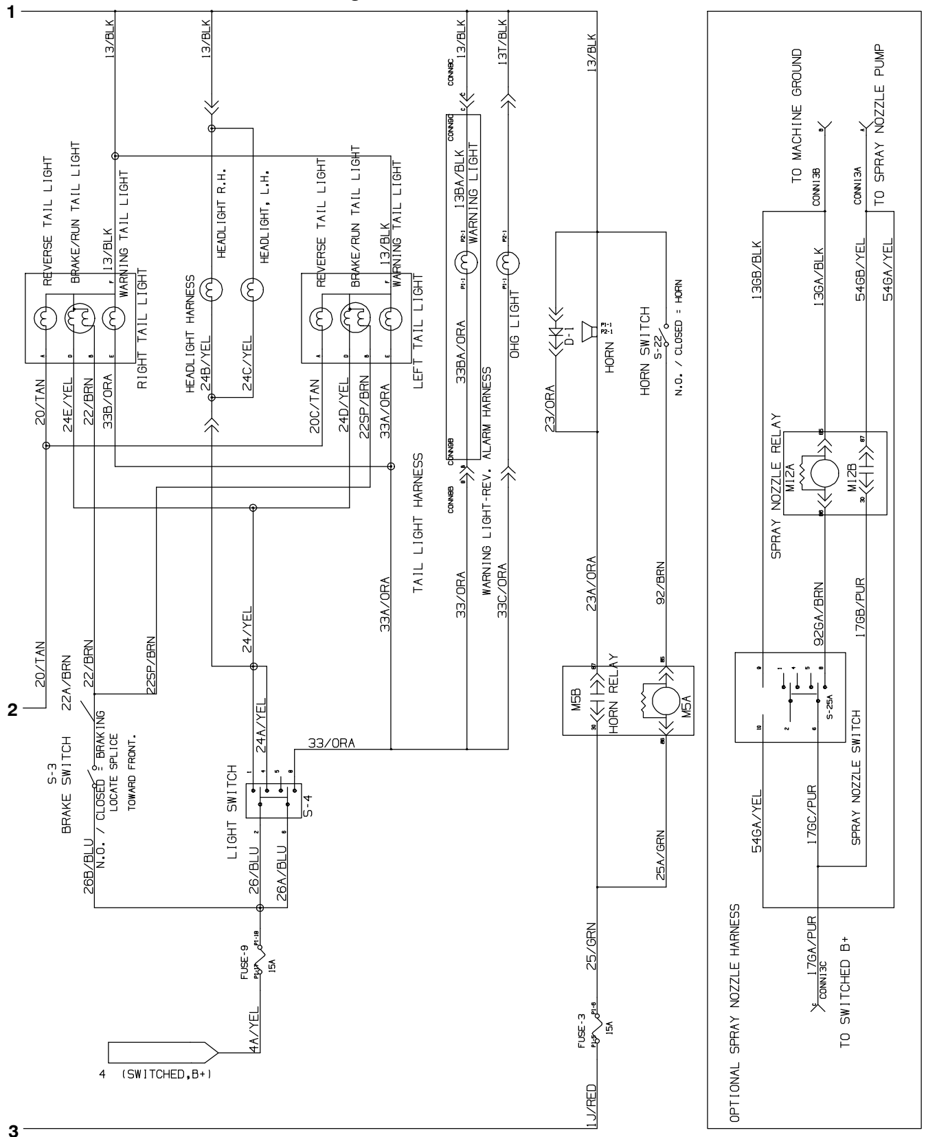
Fig. 62 – Electrical Schematic
