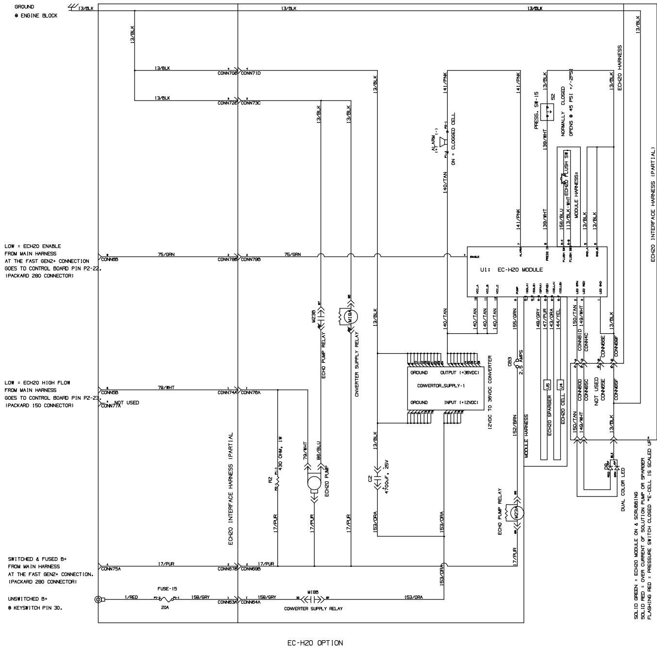
Fig. 62 – Electrical Schematic
