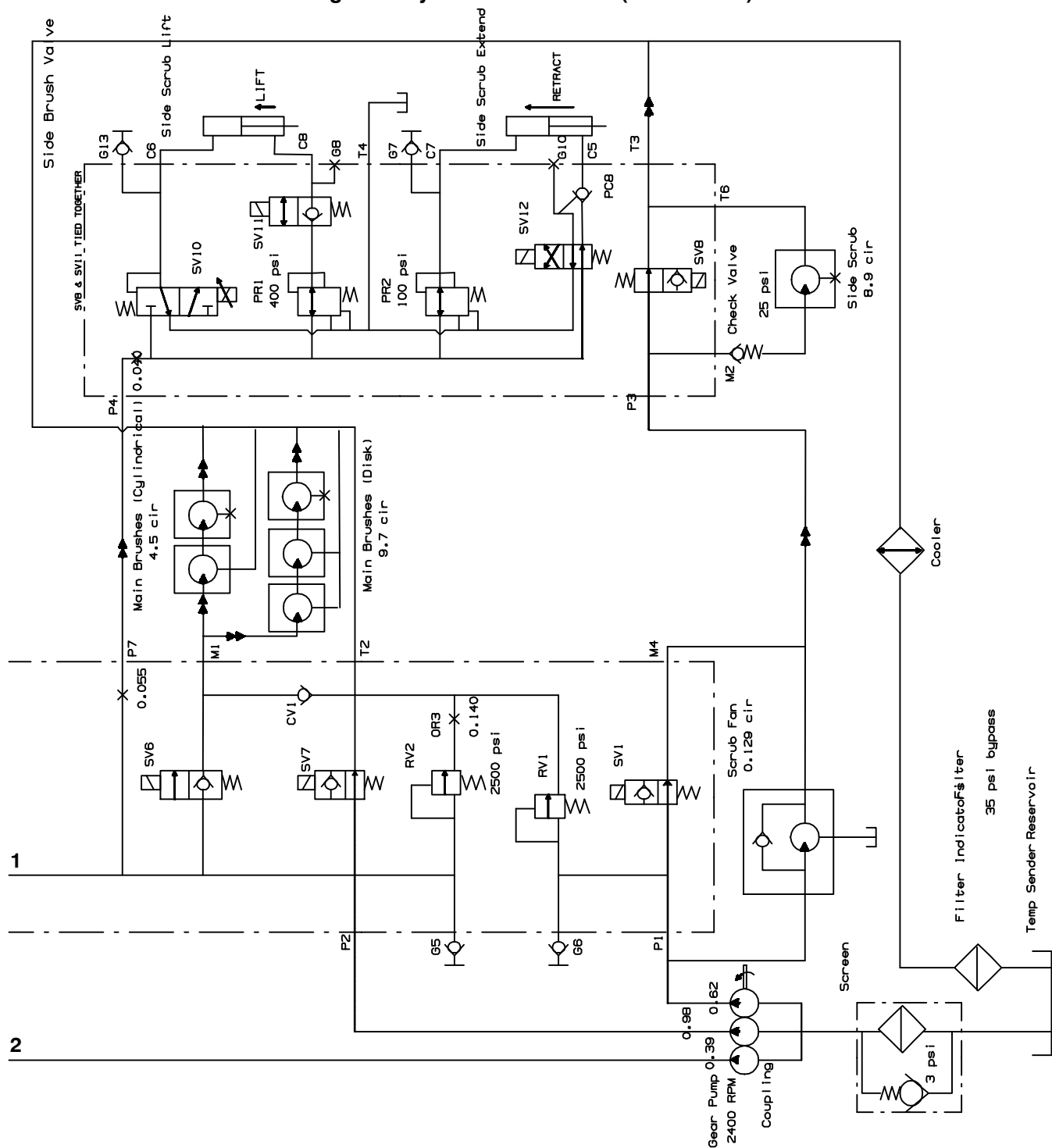
Fig. 52 – Hydraulic Schematic (0245- )
