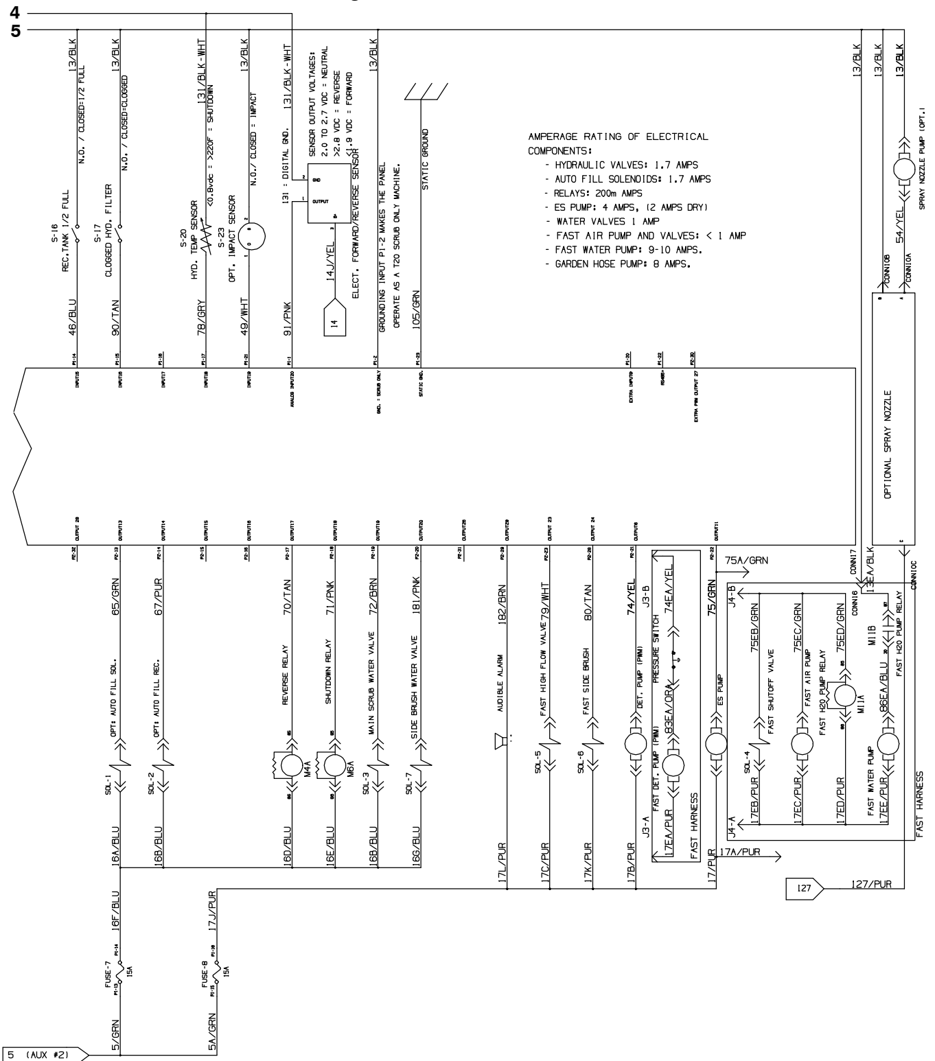
Fig. 62 – Electrical Schematic
