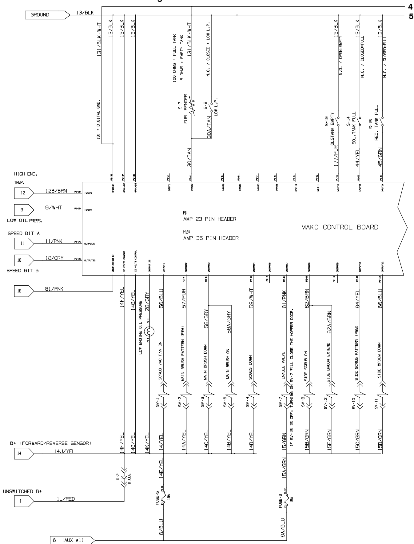
Fig. 62 – Electrical Schematic
