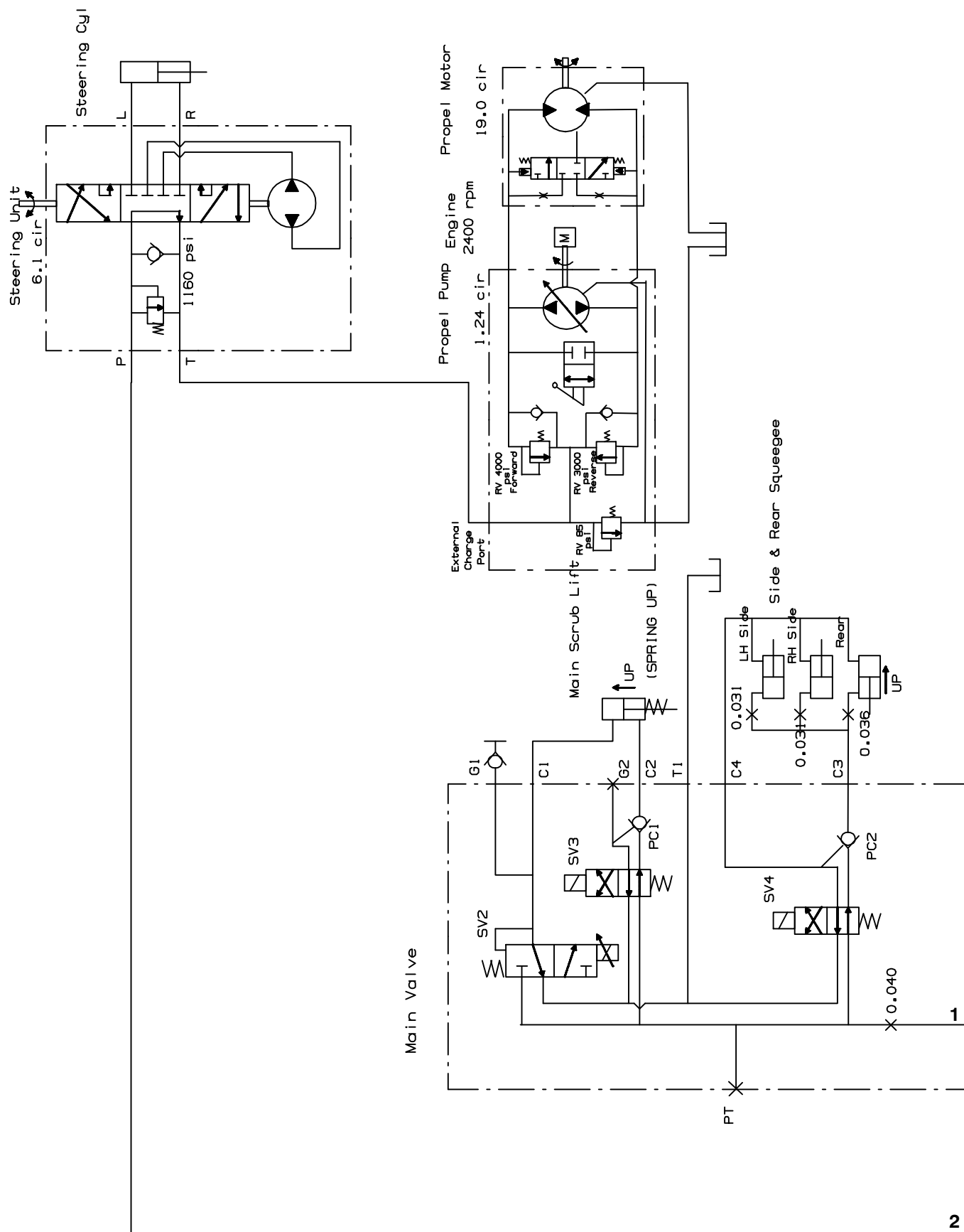
Fig. 51 – Hydraulic Schematic (0043–0244)
