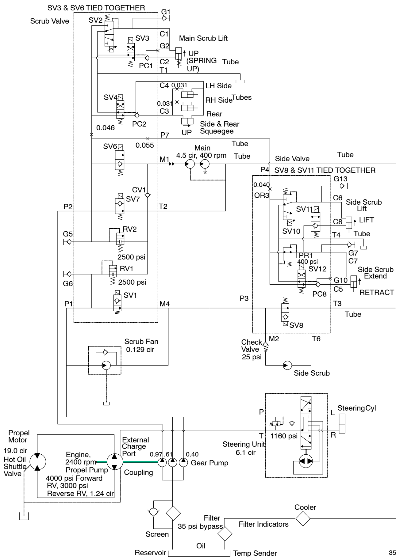
Fig. 71 – Hydraulic Schematic (0000–0042)
