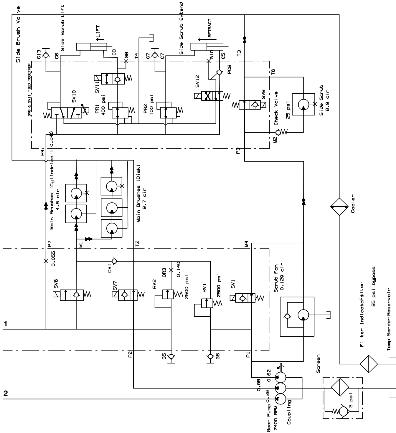
Fig. 73 – Hydraulic Schematic (0245– )
