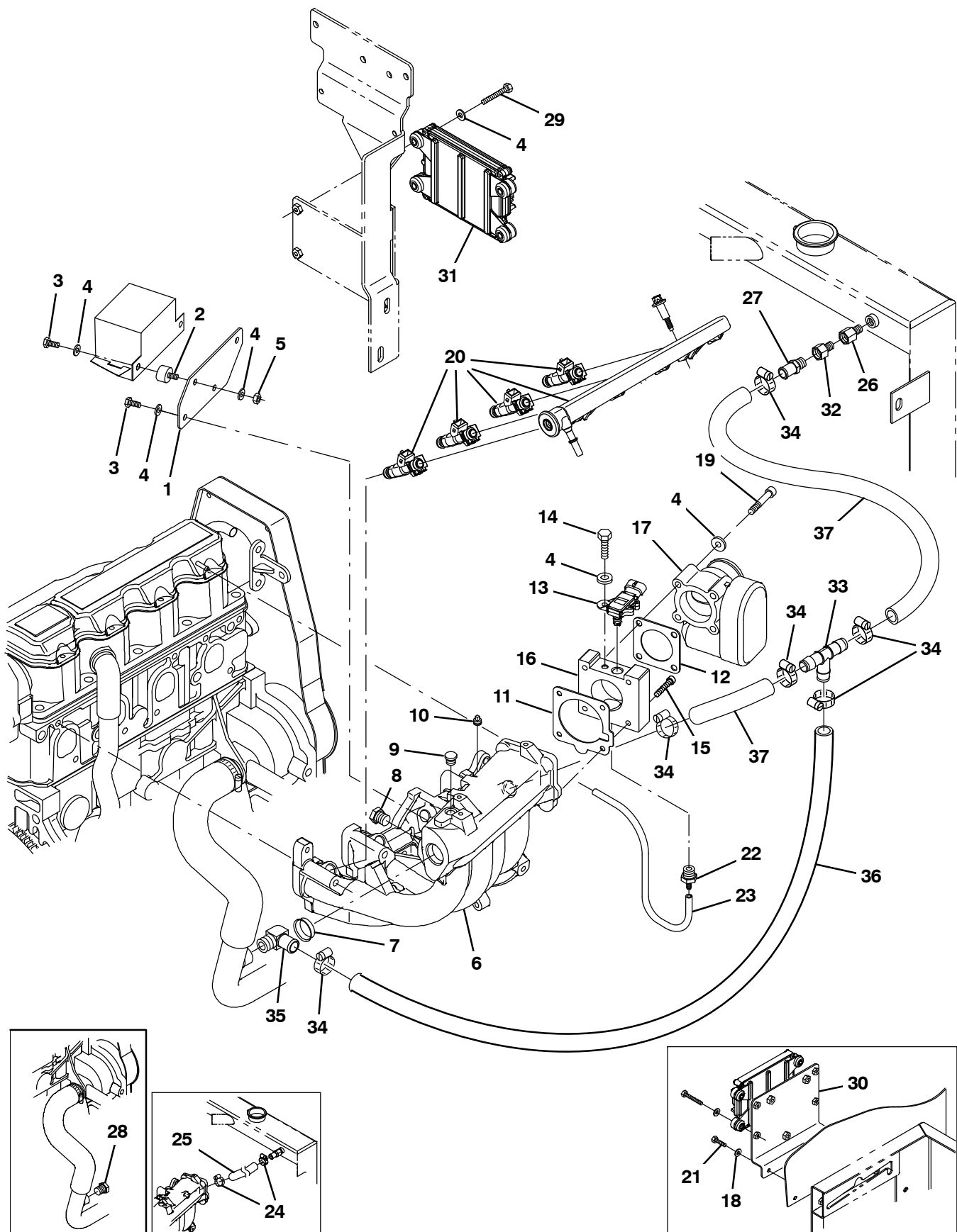
Fig. 14 – GM Engine EFI Group, Gasoline (0203–0499)
