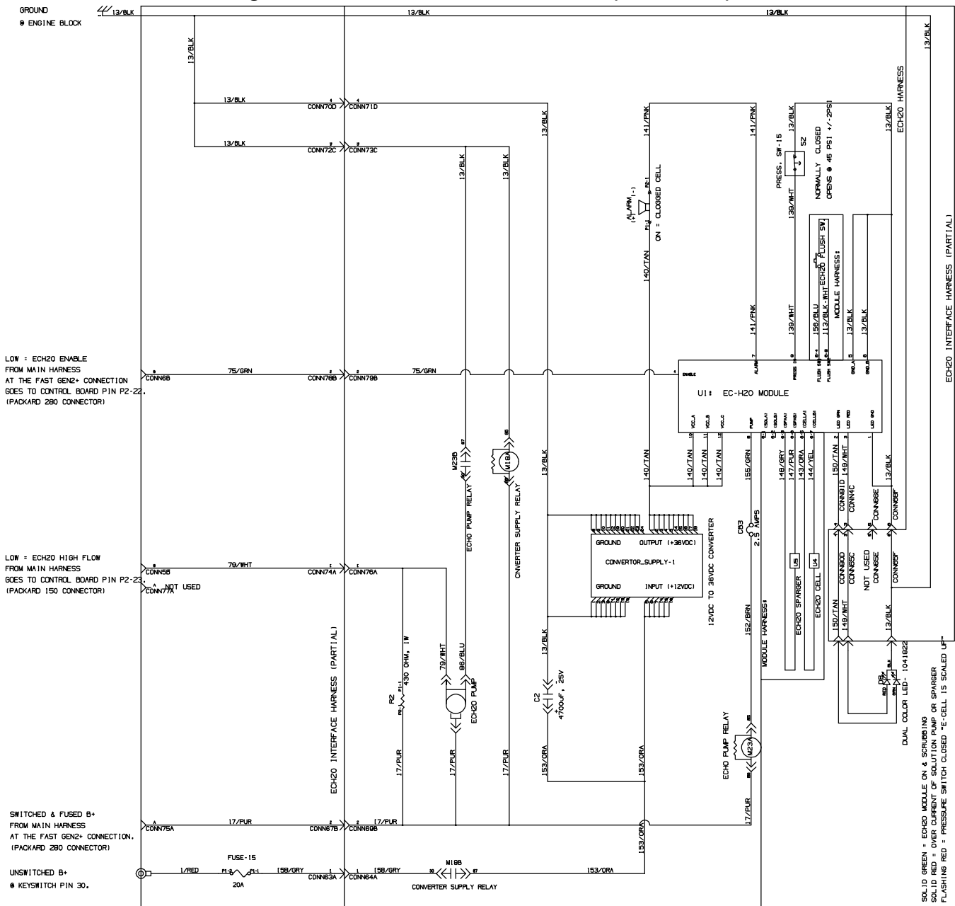
Fig. 91 – Mitsubishi Electrical Schematic (0500– )
