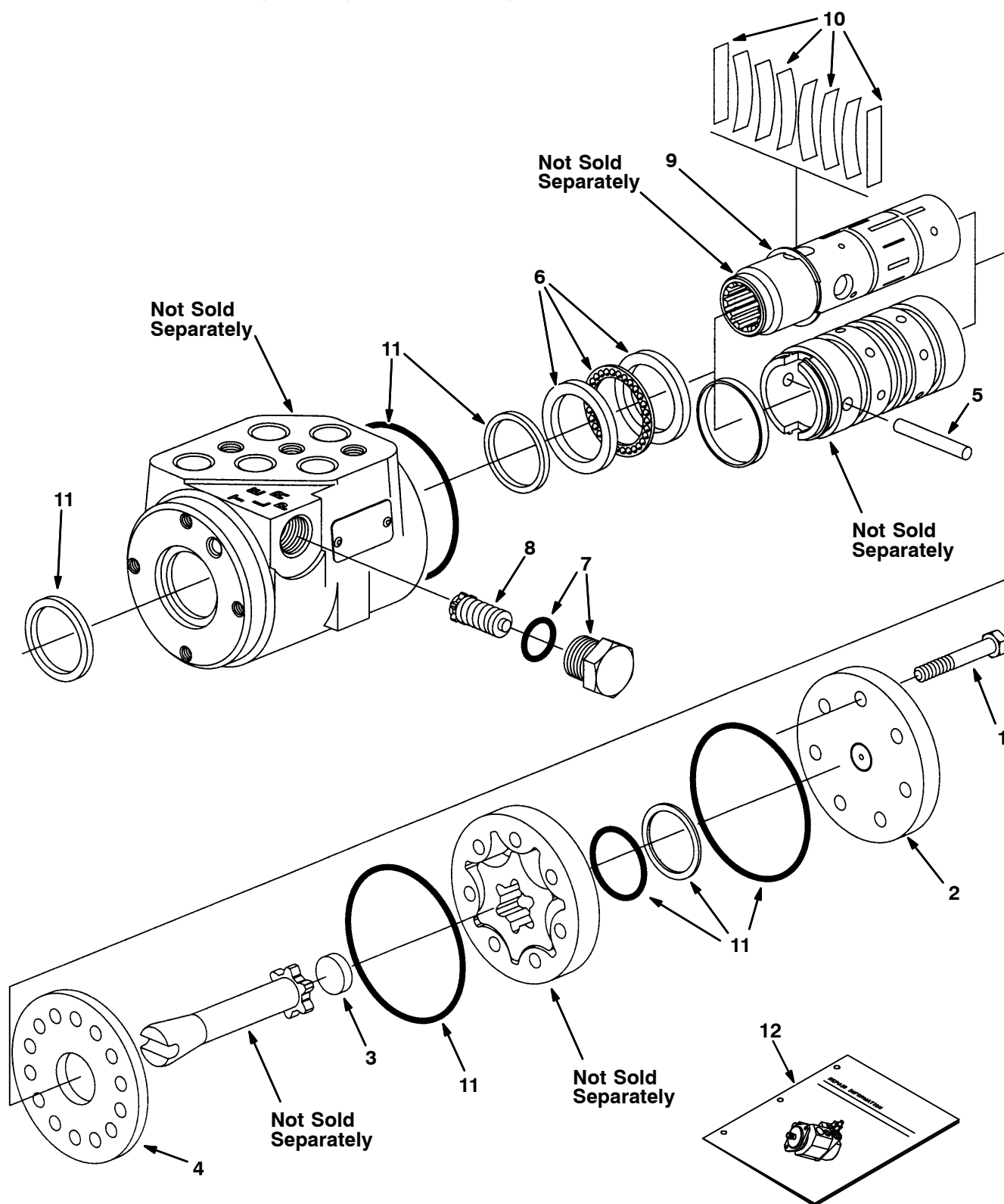
Fig. 13 – Hydraulic Steering Valve Breakdown, 1024260
