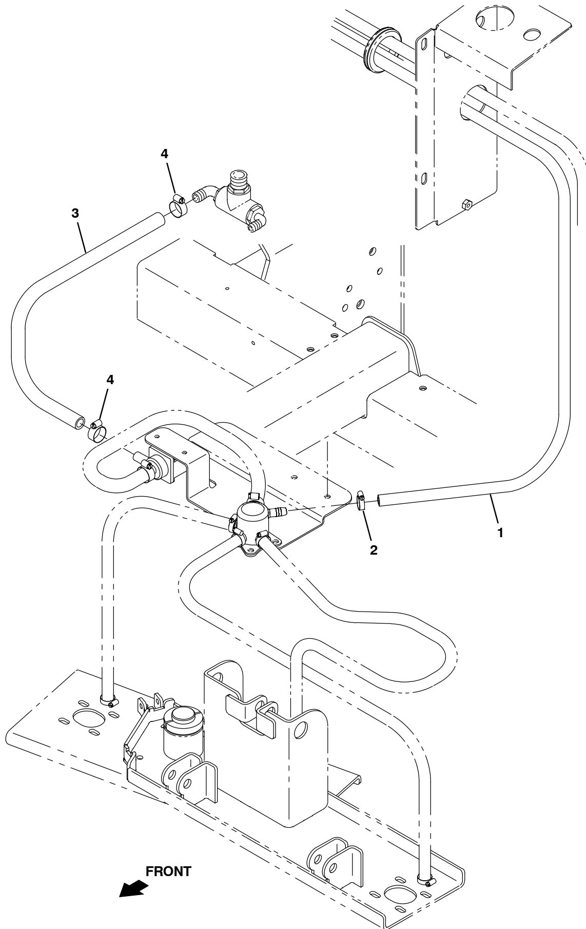
Fig. 26 – ec-H2O Solution Supply Group, Disk Scrub Head
