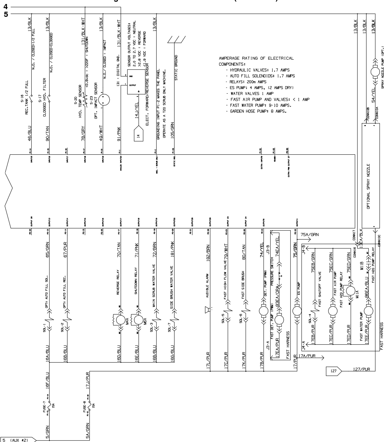
Fig. 83 – GM Electrical Schematic (0000–0043)
