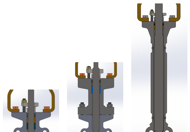
Figure 7: Standard bonnet
