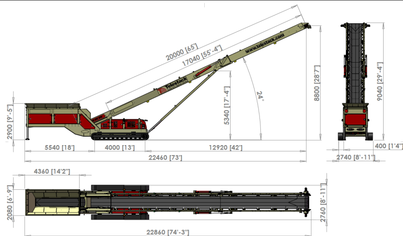
24° - FULLY RAISED
