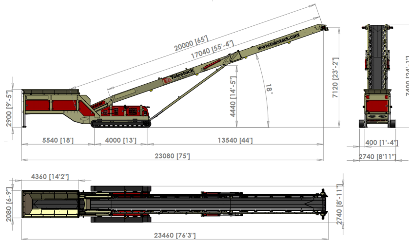
18° - OPERATIONAL
