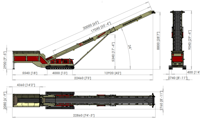
24° - FULLY RAISED
