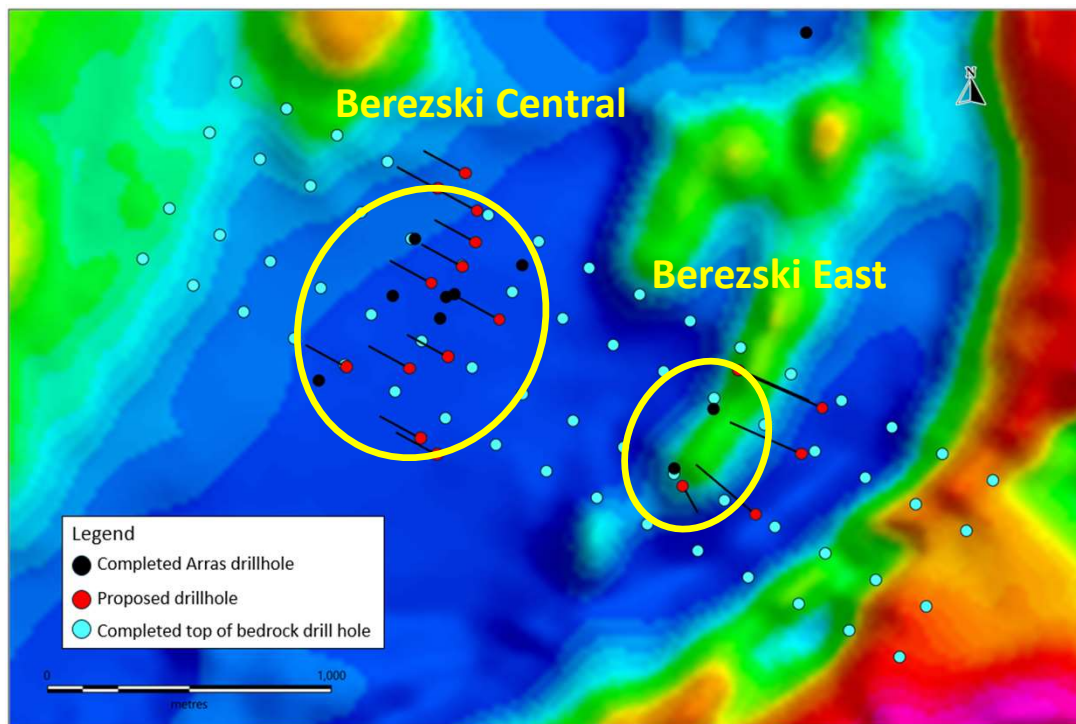
Plan map showing completed and proposed diamond drill-holes and completed top of bedrock drillholes, Berezski Central and Berezski East targets overlain on RTP airborne magnetic data.
