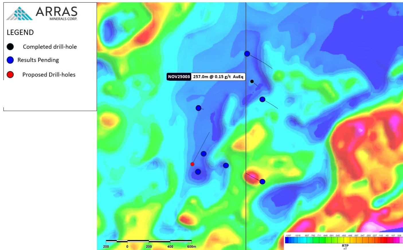
Novii Target showing completed and planned drill-holes overlain on ground magnetic data (reduced to pole)
