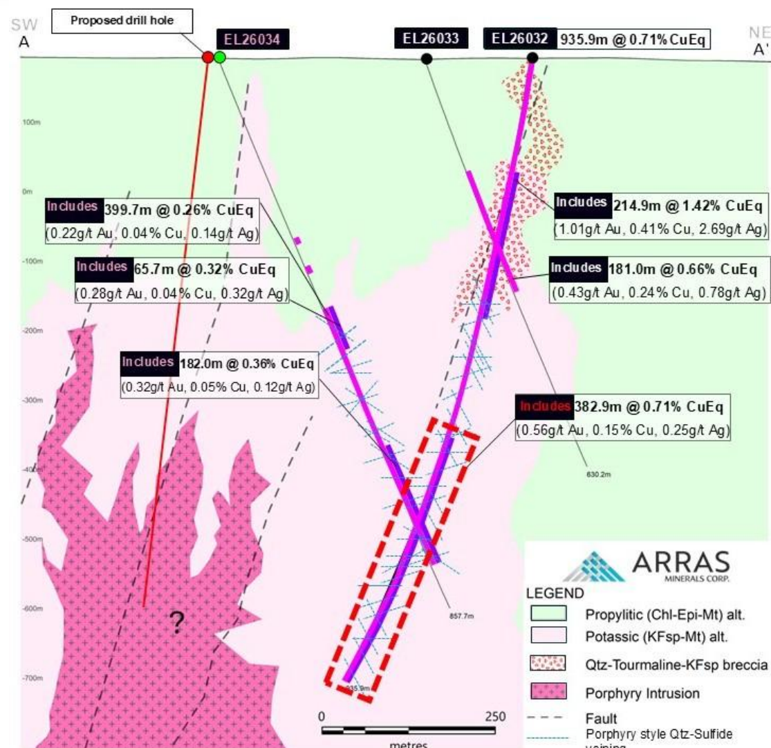
Long section through the Berezski North target showing Arras drill-hole intercepts, including EL26034. Mineralization and potassic alteration increase with depth in EL26032 as the hole drills toward the interpreted intrusive porphyry centre, whereas mineralization and alteration decrease with depth in EL26034 as the hole drills away from the interpreted intrusion.
