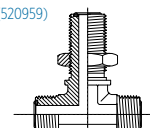
FS2703* MFS-MFS-MFS Bulkhead Tee
