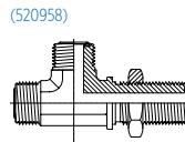
FS2704* MFS-MFS-MFS Bulkhead Tee
