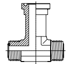
FS1805 MFS-MFS- Flange Tee Code 62
