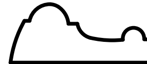
CR-6 CHAIR RAIL 1-7/16 X 3-7/16
