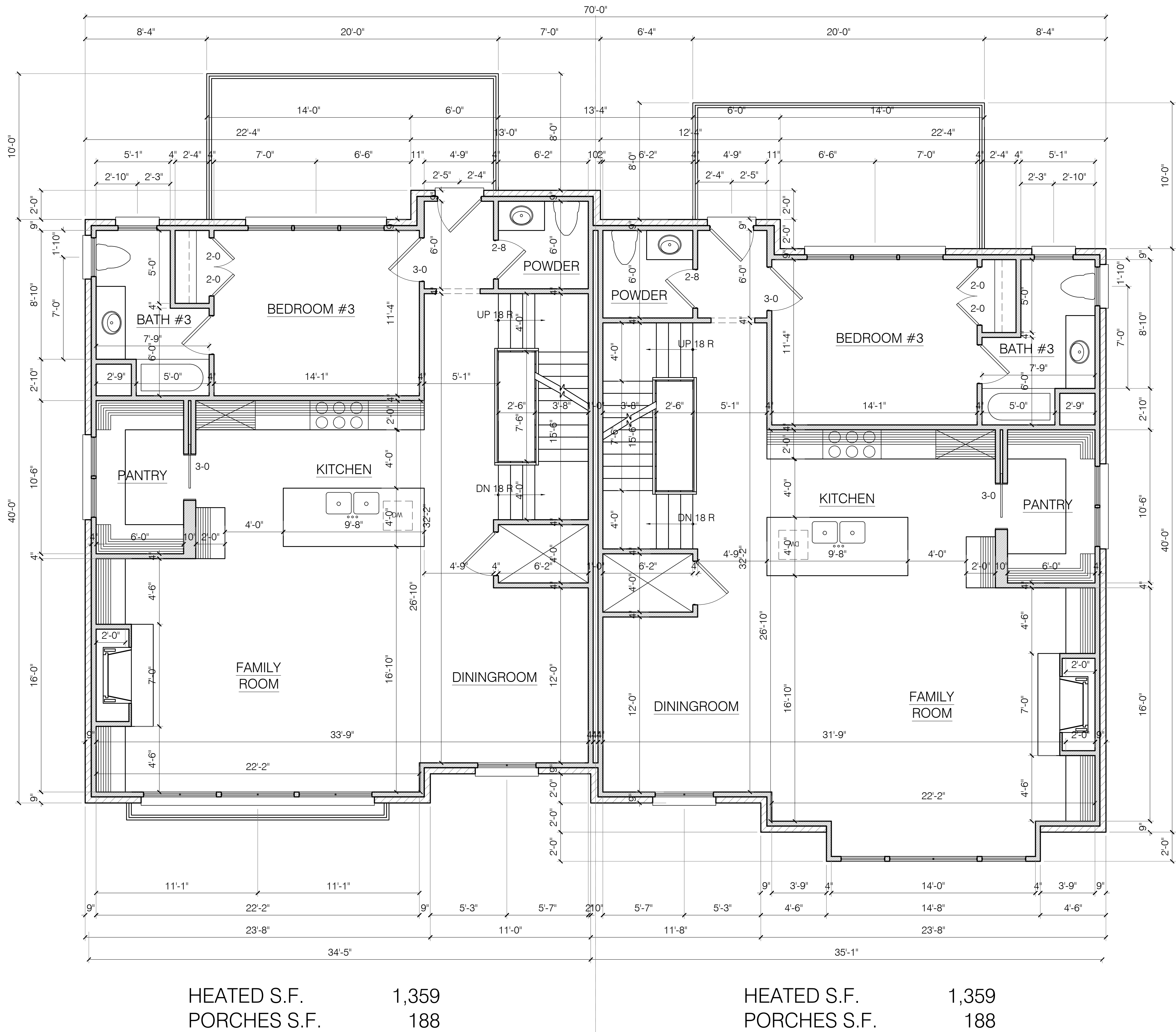
BUILDING B - SECOND FLOOR PLAN
