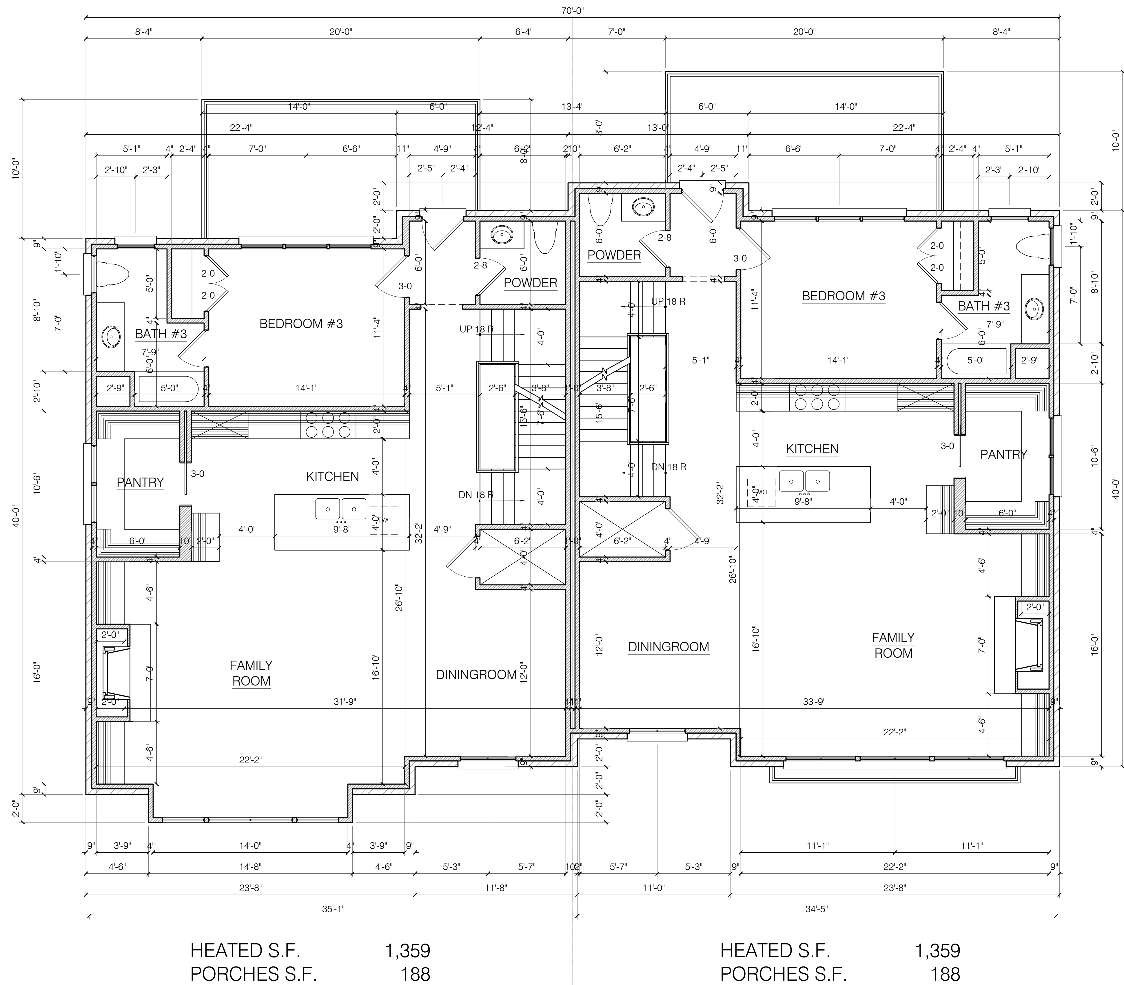
BUILDING A - SECOND FLOOR PLAN
