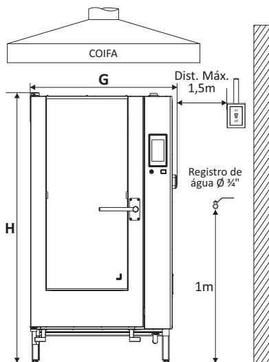
VISTA FRONTAL
