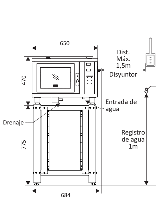
Vista Frontal
