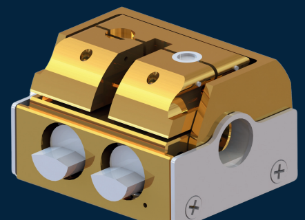
Horizontal Freeze-Fracture HPF 3.0mm holder with shutter
