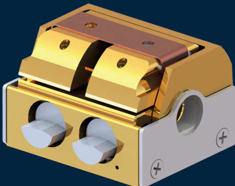
Horizontal Freeze-Fracture HPF 3.0mm holder with shutter & FLAT cover
