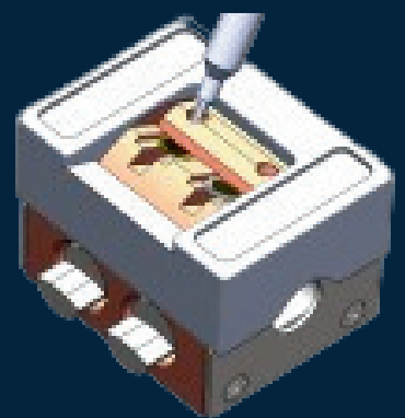
PreTilted28°ReverseEdgeClamp TEM grid holder with shutter & cold trap
