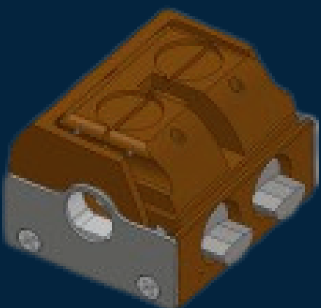
Horizontal Freeze-Fracture HPF 6.0mm holder with shutter
