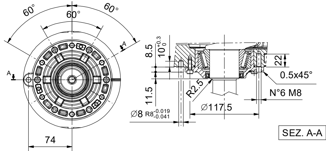
DETAIL "X" - Scale 1:2
