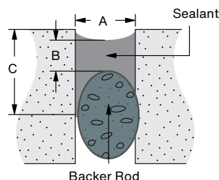
FIGURE 1: Regulates the Sealant Bead Depth
