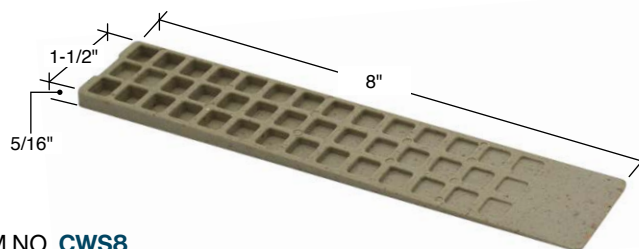
ITEM NO. CWS8 288 Shims Per Box Minimum Order: 1 Box.
