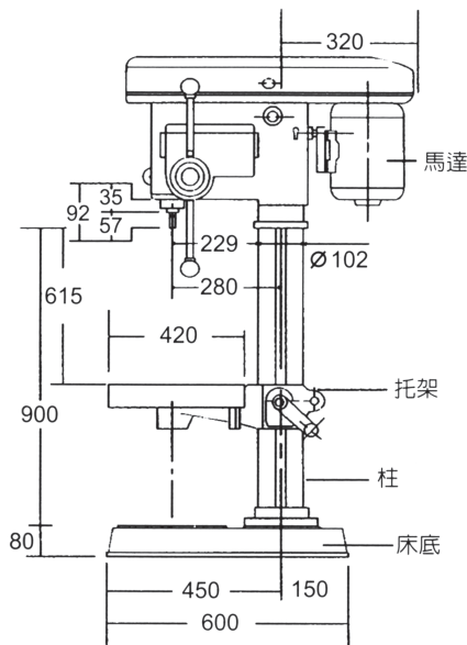
◀ TD-250 TD-25 TDT-25 TDT-32 Appearance Dimensions
