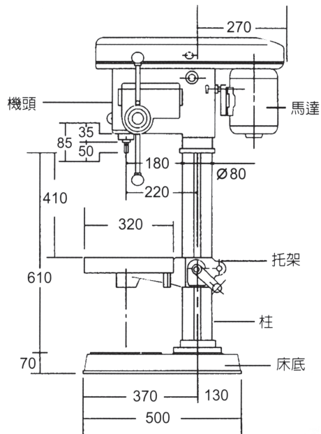
◀ TD-120 TD-14 TDT-340 Appearance Dimensions
