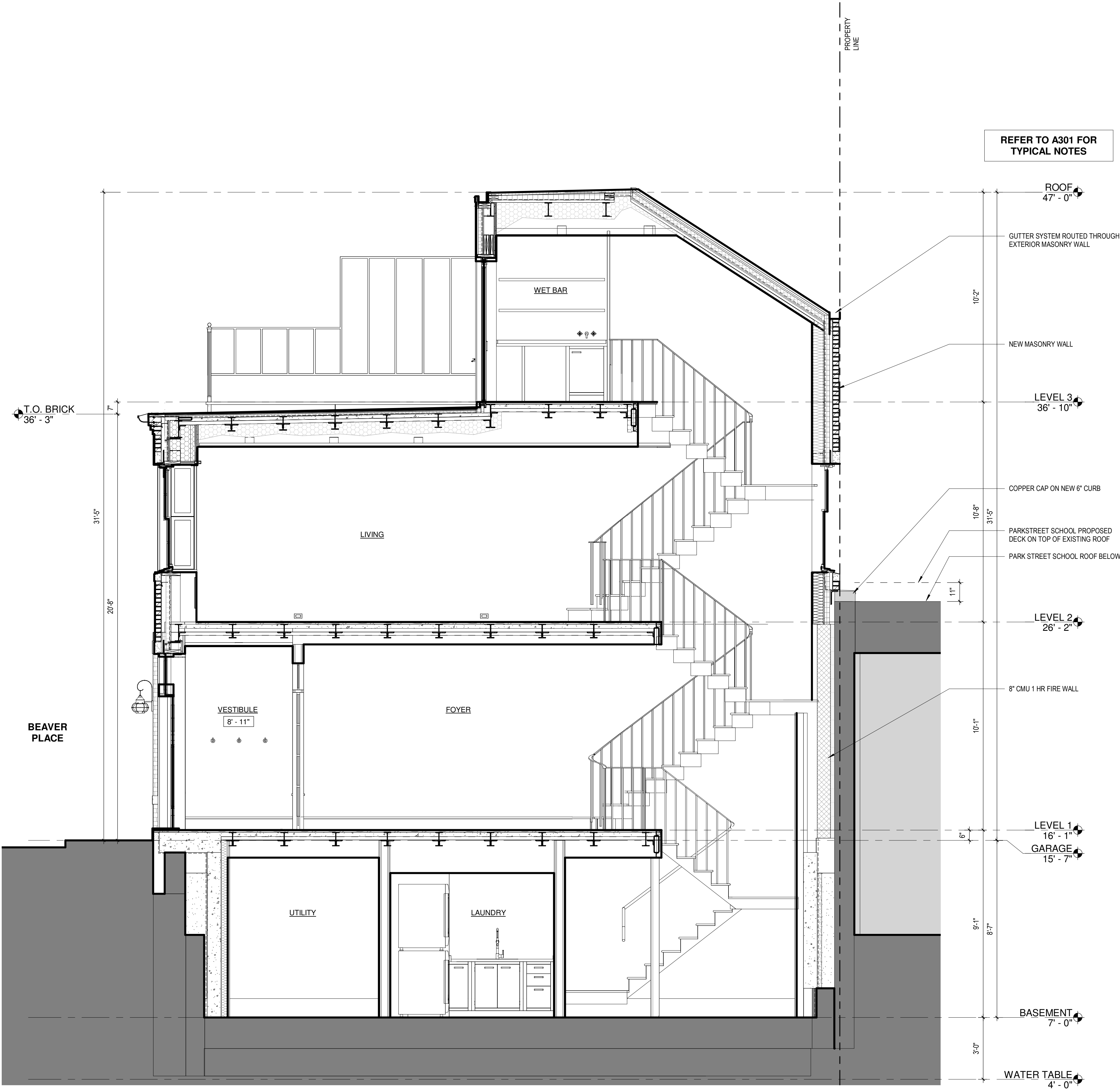
1 BUILDING SECTION 3/8" = 1'-0"
